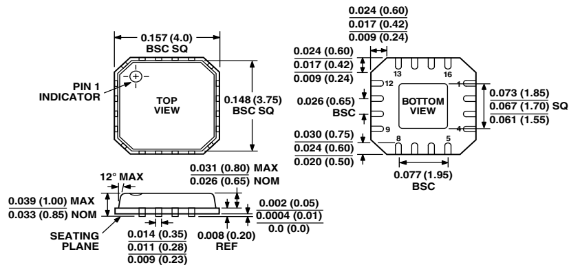
16-Terminal Leadless Frame Chip Scale (CP-16)
