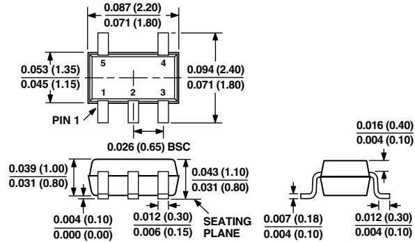
5-Lead Plastic Surface-Mount (KS-5)
