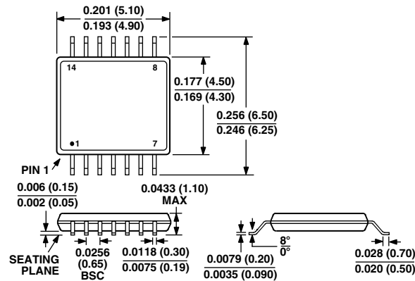
14-Lead Thin Shrink SO (RU-14)
