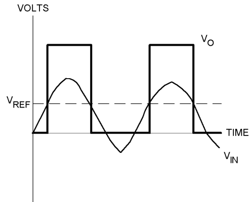
FIGURE 2. LMV7291 Basic Comparator
