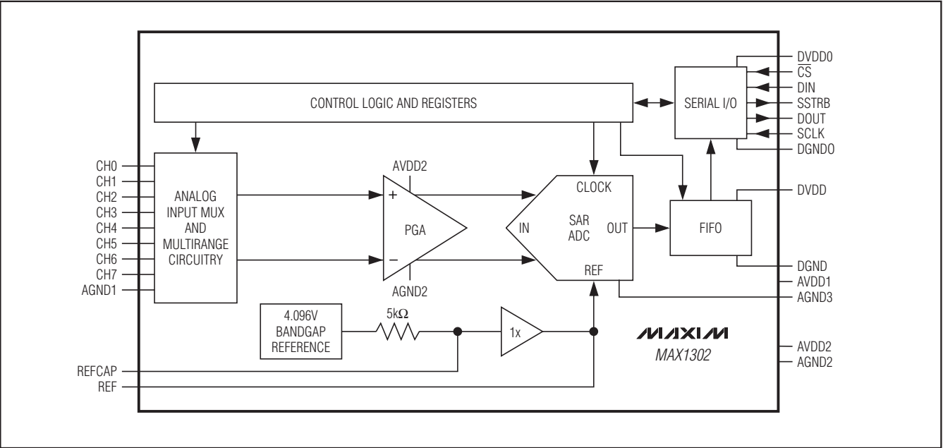
Block Diagram
