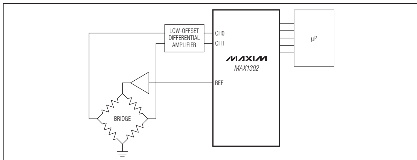
Figure 20. Bridge Application
