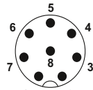
Plug, 8-pos.
