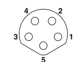
Socket, 5-pos., DeviceNet™, B-coded
