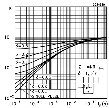
Figure 2. Thermal impedance
