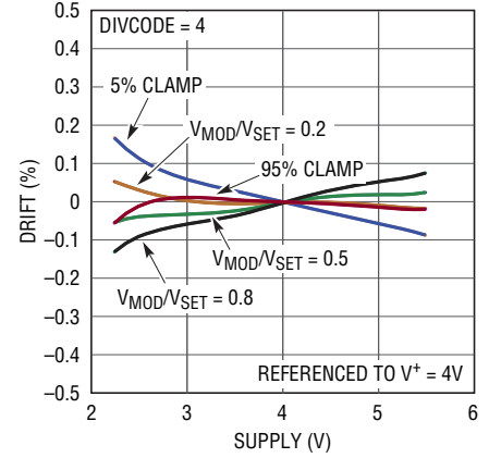
N_{DIV} > 1 Duty Cycle Drift vs Supply
