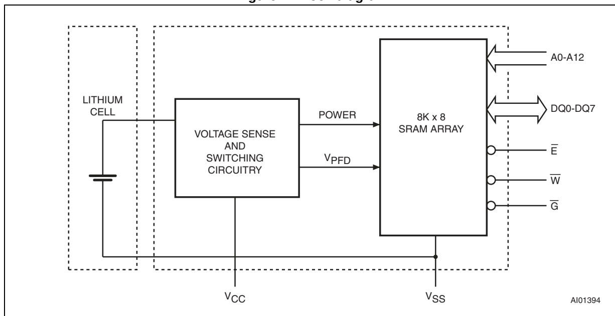
Figure 4. Block diagram
