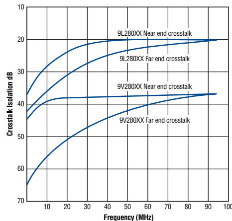
Figure 3: Balanced Crosstalk
