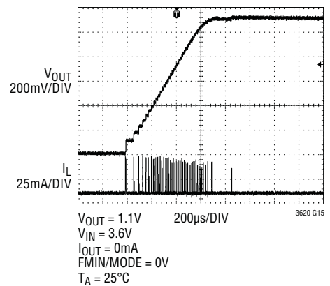
Start-Up Waveforms
