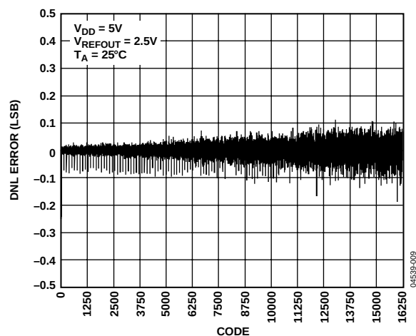
Figure 9. DNL—AD5640-2/AD5640-3
