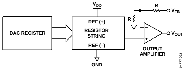
Figure 38. DAC Architecture
