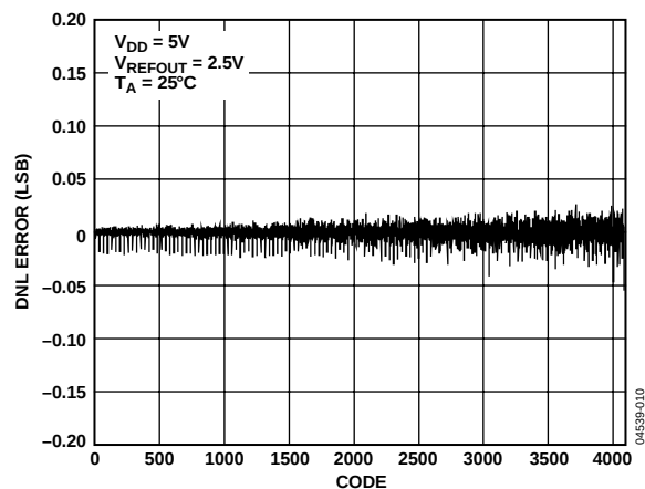
Figure 10. DNL—AD5620-2/AD5620-3
