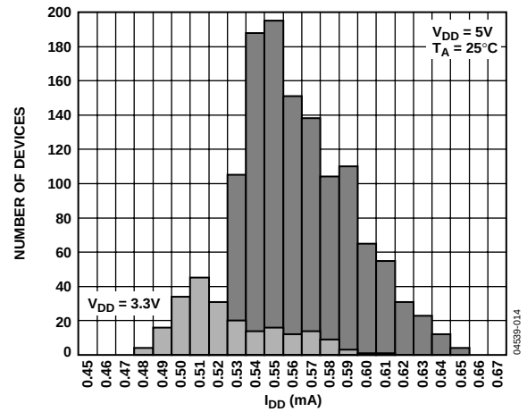
Figure 20. I_{DD} Histogram
