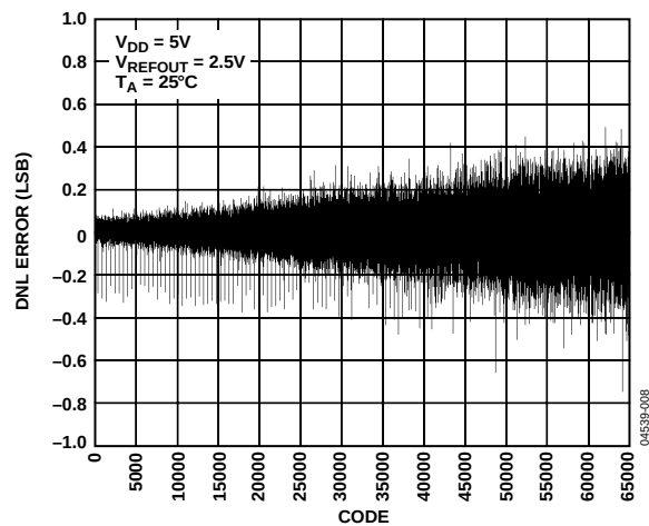
Figure 8. DNL—AD5660-2/AD5660-3
