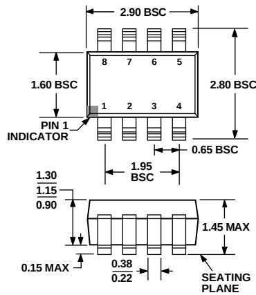
Figure 53. 8-Lead Small Outline Transistor Package [SOT-23] (RJ-8)
