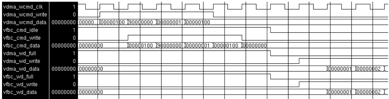
Figure 6: Write Command Interface, Write Command
