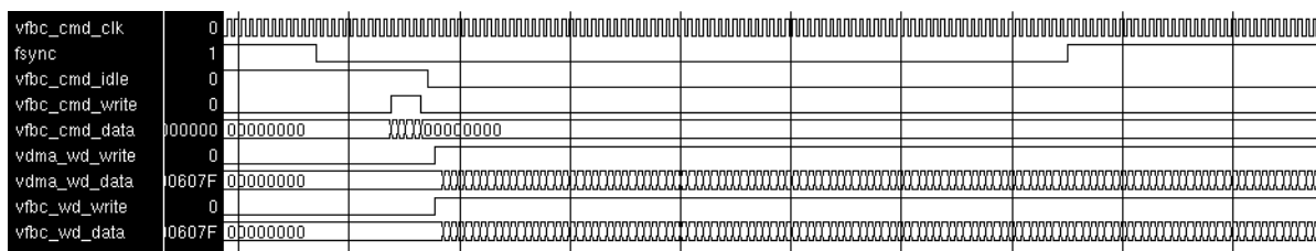
Figure 11: Write Register Command Mode Synchronized to Fsync
