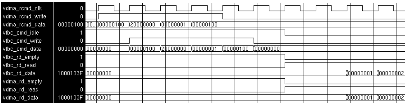
Figure 7: Read Command Interface, Read Command
