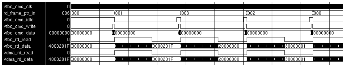
Figure 10: Gen-Lock Slave Register Read Command Mode
