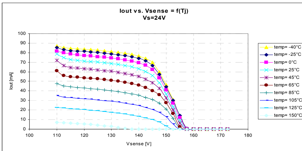
Figure 11 I_{out} vs V_{sense} = f(T_J) at V_s = 24 V
