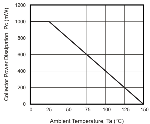
Fig.7 - P_C - T_a
