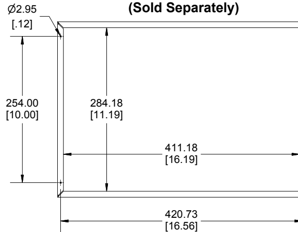
Bottom View of Chassis (Sold Separately)
