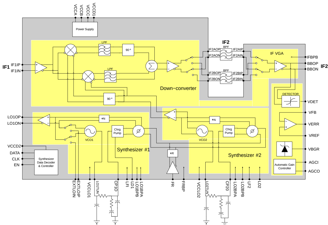
Figure 1. Detailed Block Diagram of TRF1112 / TRF1212
