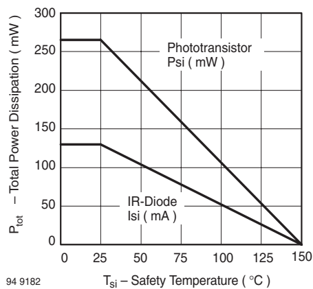
Fig. 1 Derating diagram
