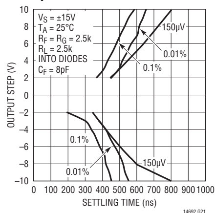
Settling Time vs Output Step, A_V = -1
