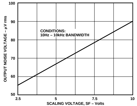
Figure 21. Wideband Noise vs. Scaling Voltage
