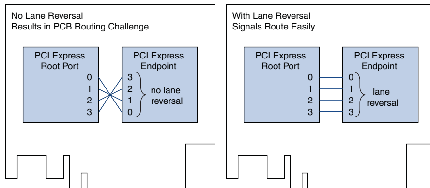
Figure 9-1. Using Lane Reversal to Solve PCB Routing Problems
