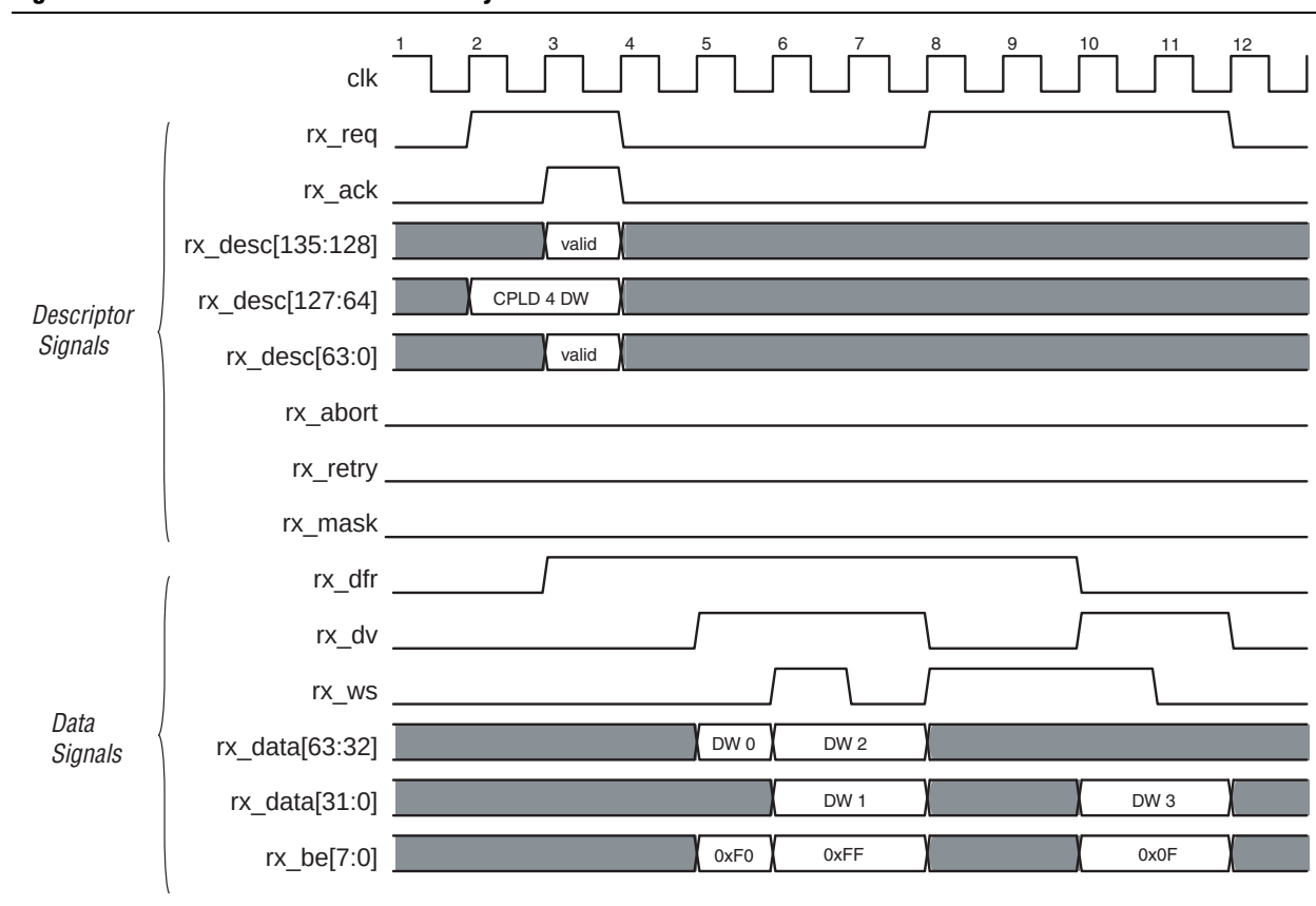
Figure B–9. RX Transaction with a Data Payload and Wait States Waveform
