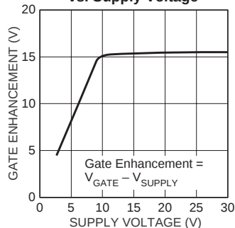
Gate Enhancement vs. Supply Voltage
