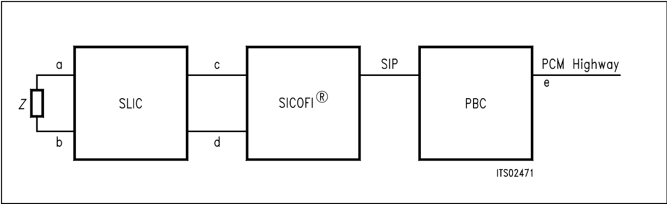
Figure 11 Definition of Transfer Functions
