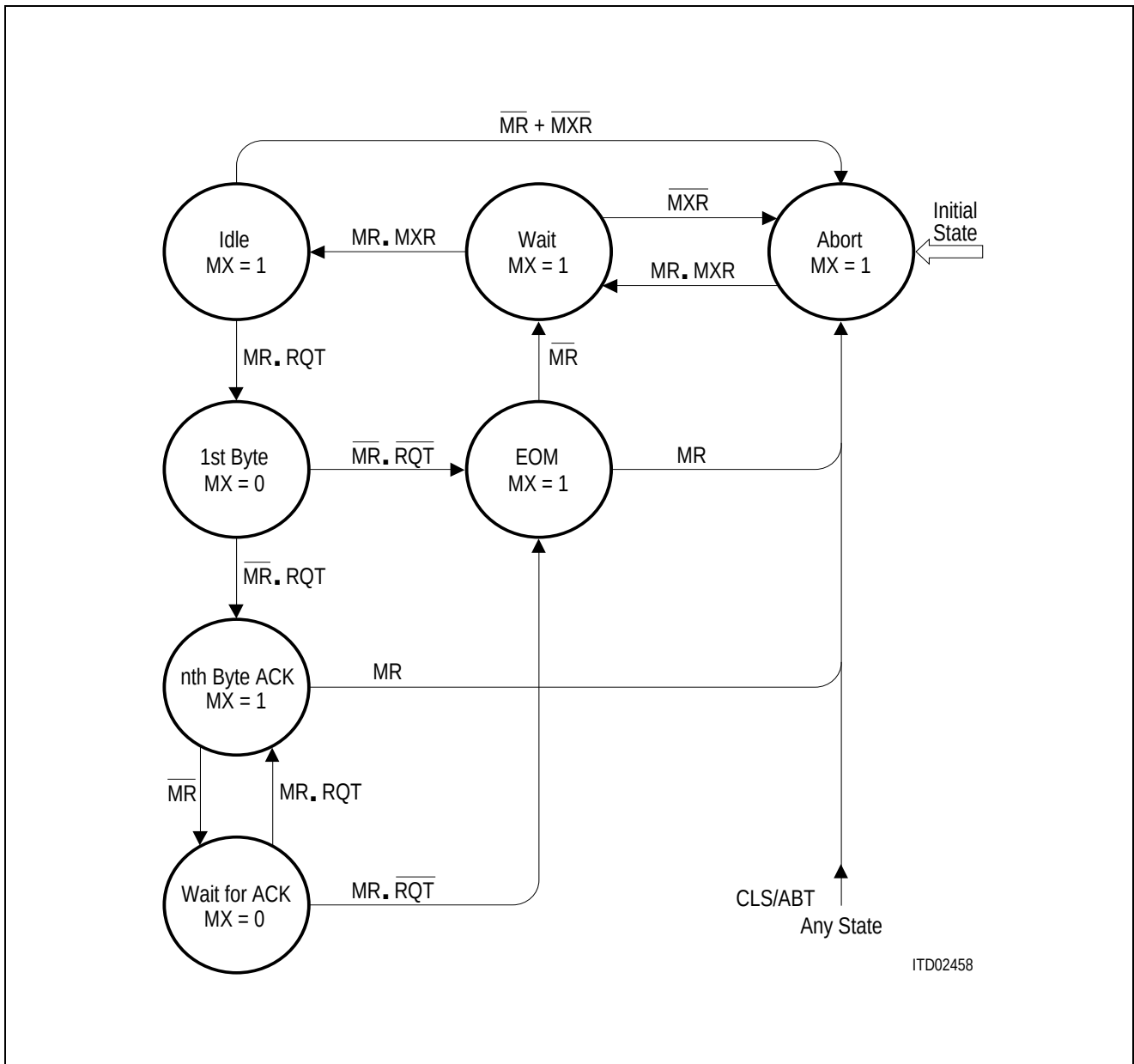
State Diagram of the SICOPI®-2 MONITOR Transmitter
