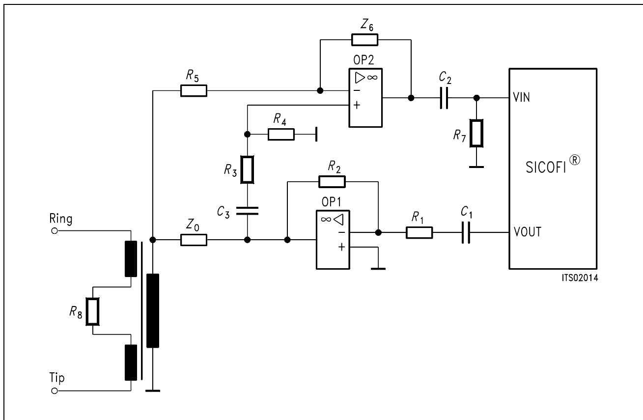
Figure 12 SLIC Circuit
