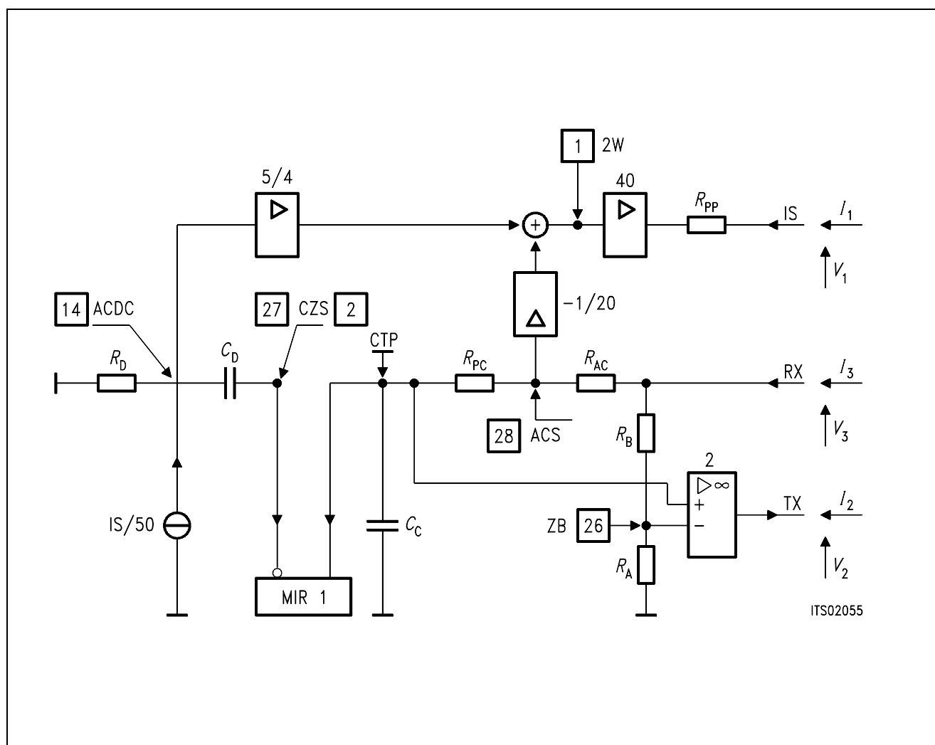
Figure 5 L3090/L3000 Model
