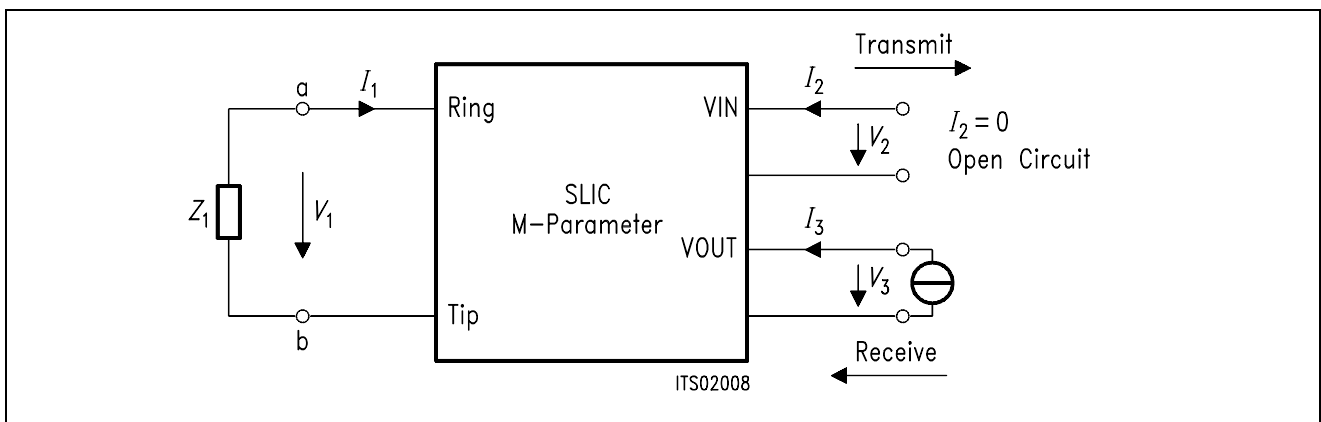
Figure 11 Definition of SLIC ZSLI
