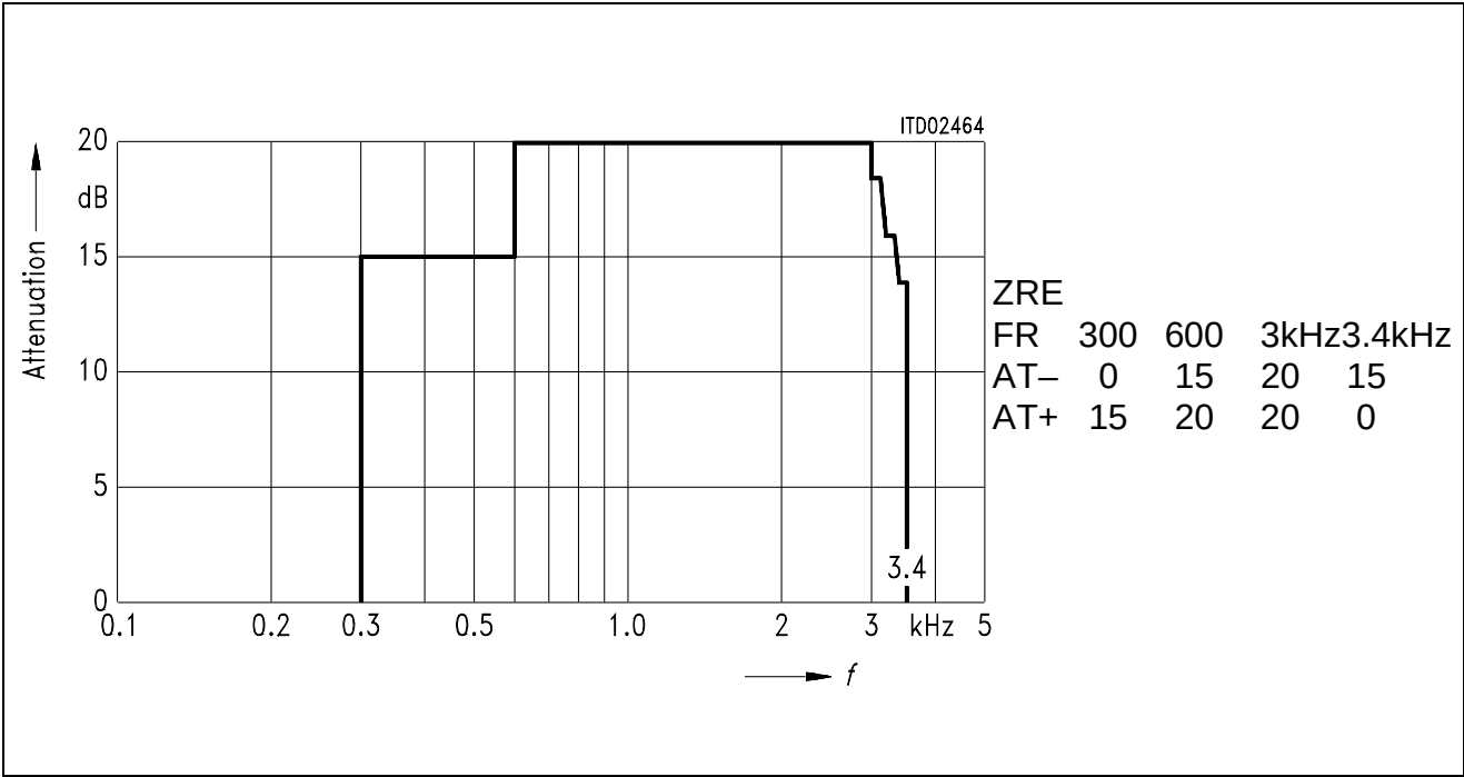
Figure 10 Specification Mask
