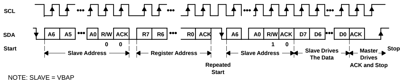
Figure 2. I²C Read From VBAP: Protocol A
