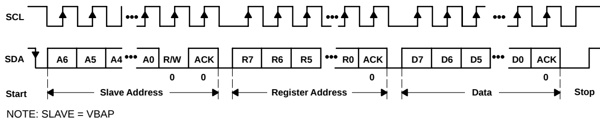
Figure 1. I²C Bus Write to VBAP
