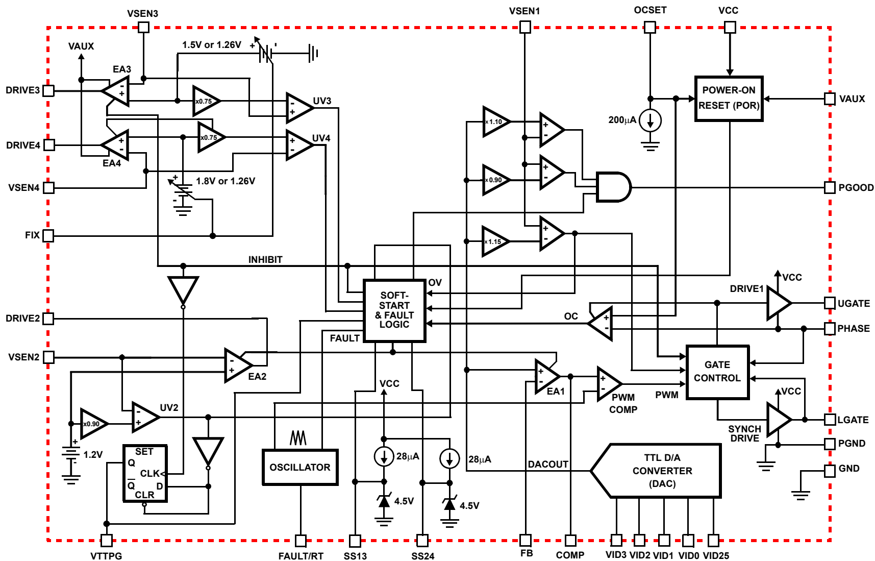
FIGURE 1. BLOCK DIAGRAM
