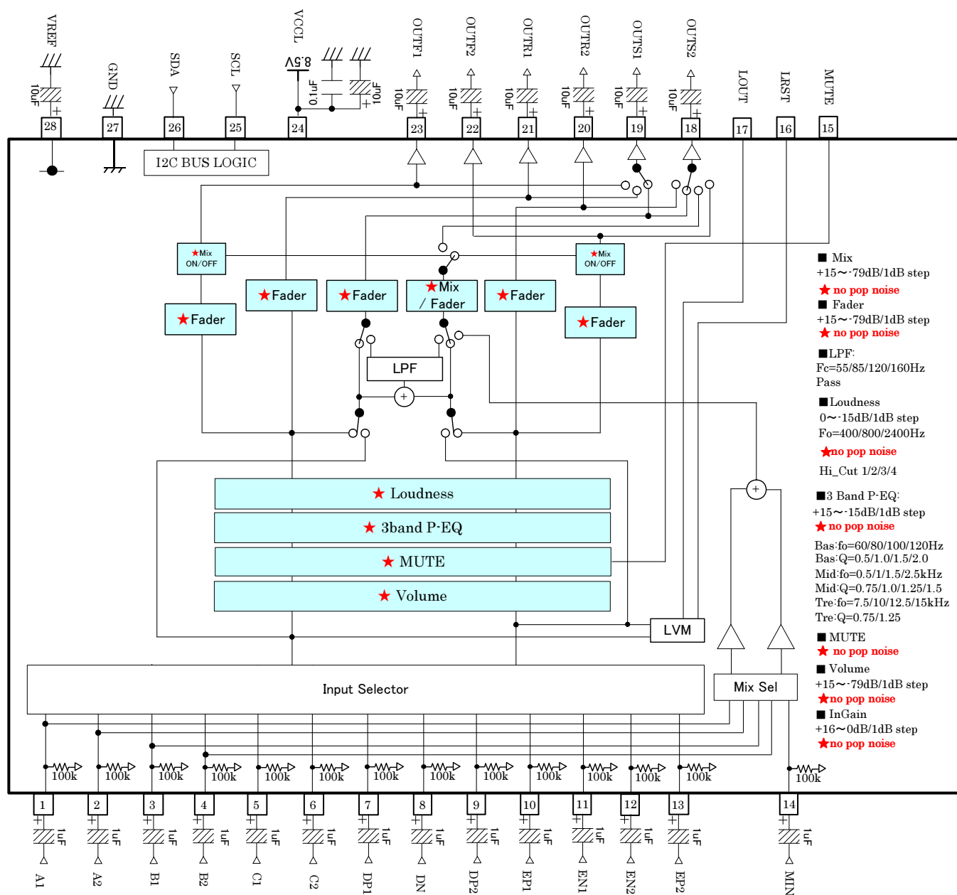
Figure 24. Application Circuit Diagram
