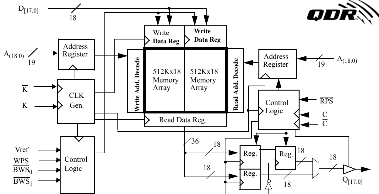
Logic Block Diagram (CY7C1303V25)
