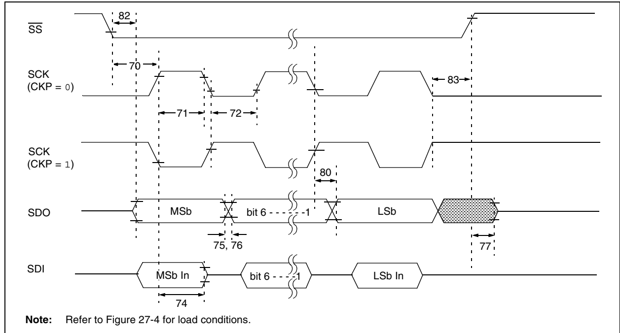
FIGURE 27-15: EXAMPLE SPI SLAVE MODE TIMING (CKE = 1)
