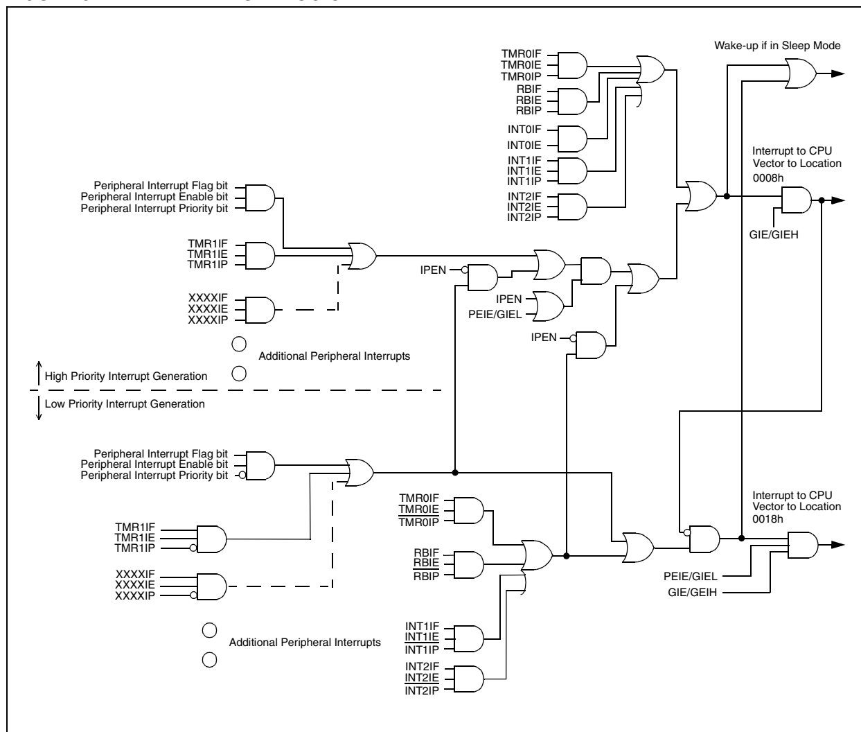
FIGURE 9-1: INTERRUPT LOGIC
