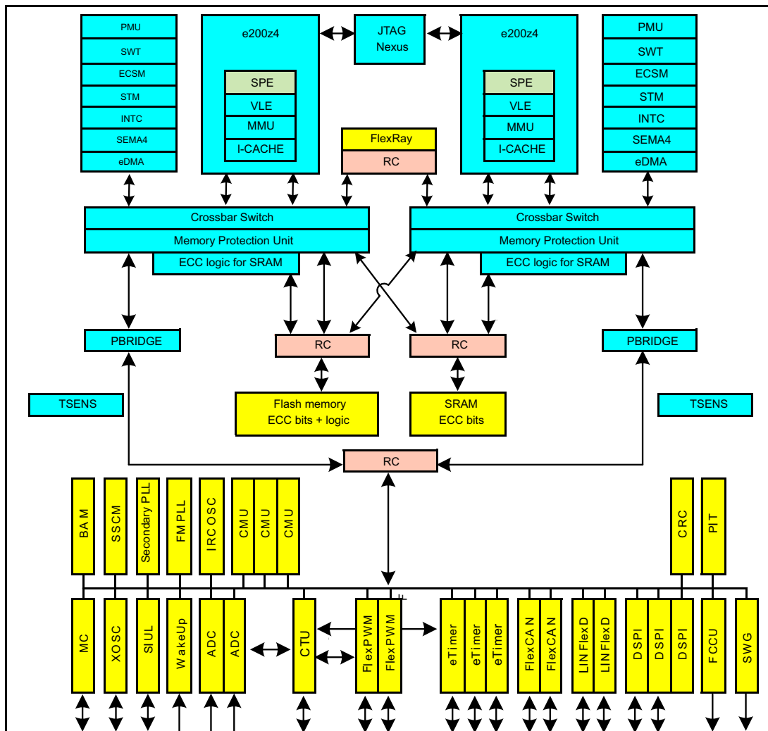
Figure 1. SPC56EL60 block diagram
