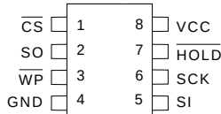
8-pin SOIC
