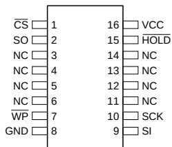
16-pin SOIC
