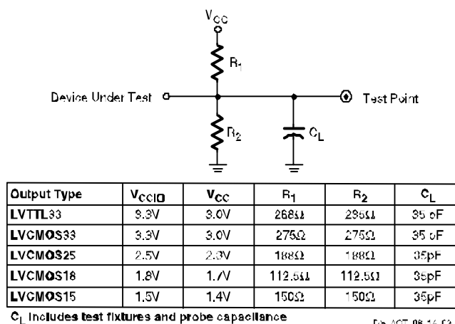
Figure 3: AC Load Circuits
