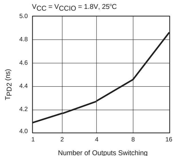
Figure 2: Derating Curve for T_{PD}
