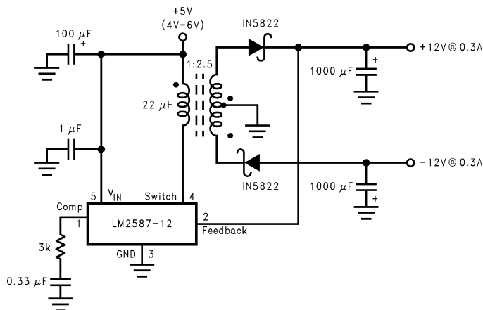
Flyback Regulator
