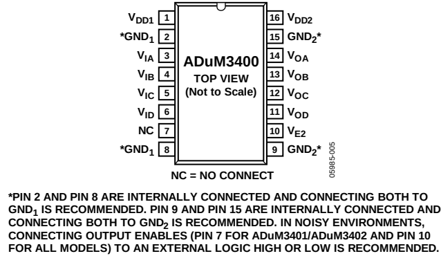
Figure 5. ADuM3400 Pin Configuration
