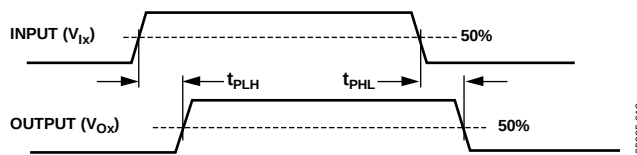
Figure 18. Propagation Delay Parameters
