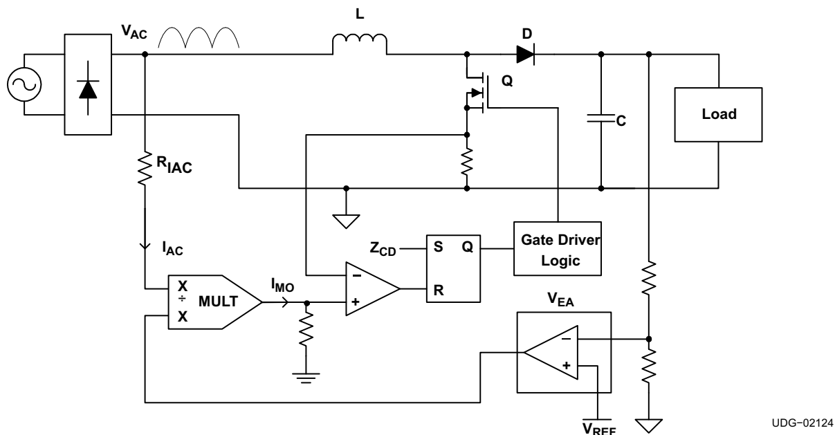
Figure 7. Basic Block Diagram of CRM Boost PFC
