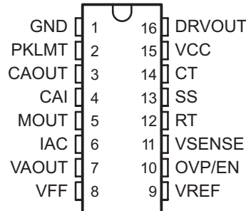
Pin Functions
