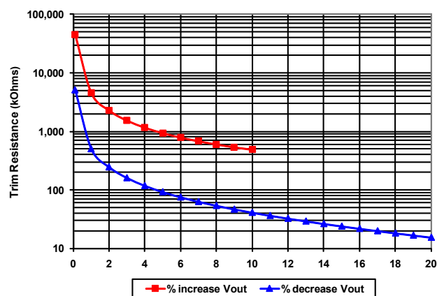
Figure C: Trim Graph
