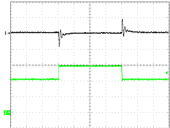
Figure 16: Output voltage response to step-change in load current (50%-75%-50% of I_{out(max)} ; dI/dt = 5A/\mu s ). Load cap: 470 \mu F , 30 mW ESR tantalum cap and 1 \mu F ceramic cap. Ch 1: Vout (200mV/div), Ch 2: Iout (5A/div).
