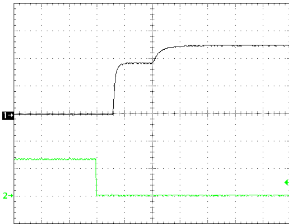
Figure 13: Turn-on transient at full load (resistive load) (5 ms/div). Input voltage pre-applied. Ch 1: Vout (2V/div). Ch 2: ON/OFF input (5V/div).
