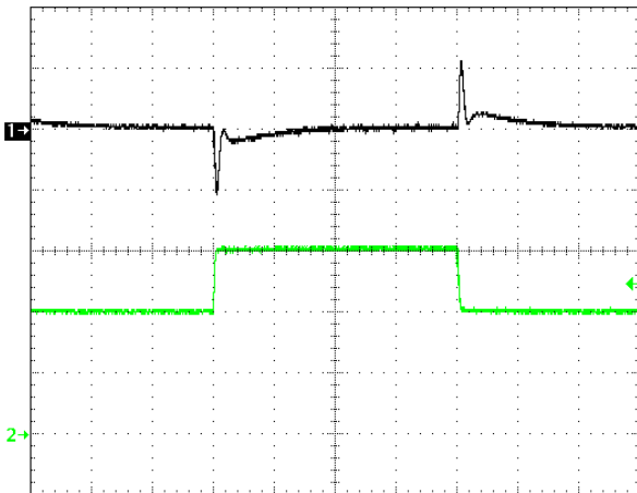
Figure 15: Output voltage response to step-change in load current (50%-75%-50% of I_{out(max)} ; dI/dt = 0.1A/\mu s ). Load cap: 10 \mu F , 100 m \Omega ESR tantalum cap and 1 \mu F ceramic cap. Ch 1: Vout (200mV/div), Ch 2: Iout (5A/div).
