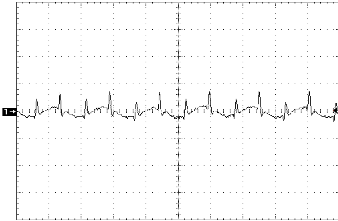
Figure 19: Input reflected ripple current, is, through a 10 \mu H source inductor at nominal input voltage and rated load current (20 mV/div). See Figure 17.
