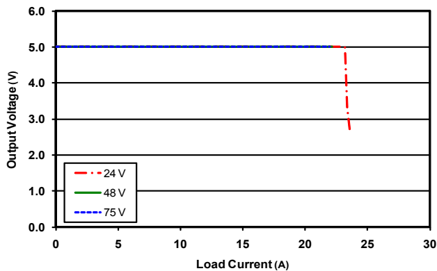
Figure 21: Output voltage vs. load current showing typical current limit curves and converter shutdown points.
