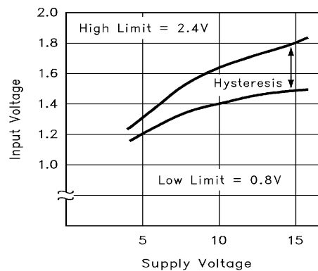
FIGURE 2. SWITCH THRESHOLD vs SUPPLY VOLTAGE
