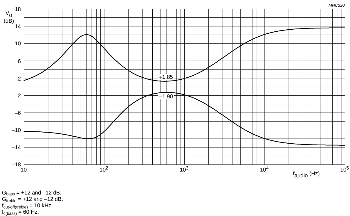
Fig.3 Equalizer bowing.
