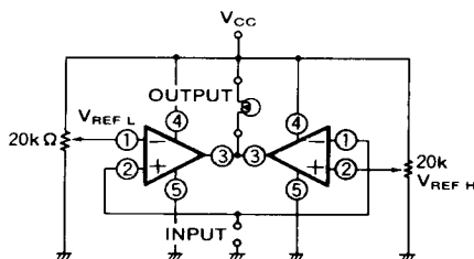
(4) Window comparator (alarm circuit)
