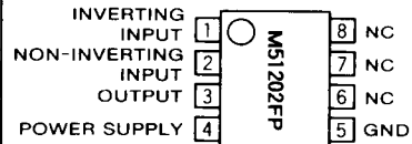
Outline 8P2S
