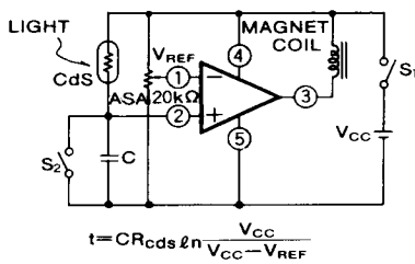
(3) Electric shutter
