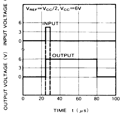
PULSE RESPONSE CHARACTERISTICS
