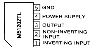
Outline 5P5T
