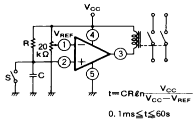
(2) CR Timer
