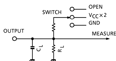
Figure 1 AC Characteristics Measurement Circuit
