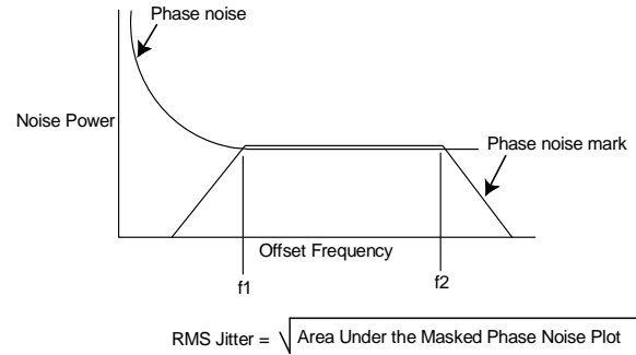
Figure 7. RMS Phase Jitter
