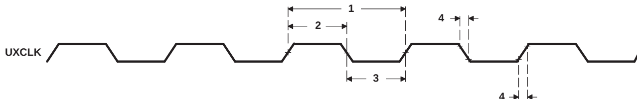
Figure 7-74. UXCLK Timing
