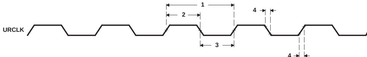
Figure 7-75. URCLK Timing
