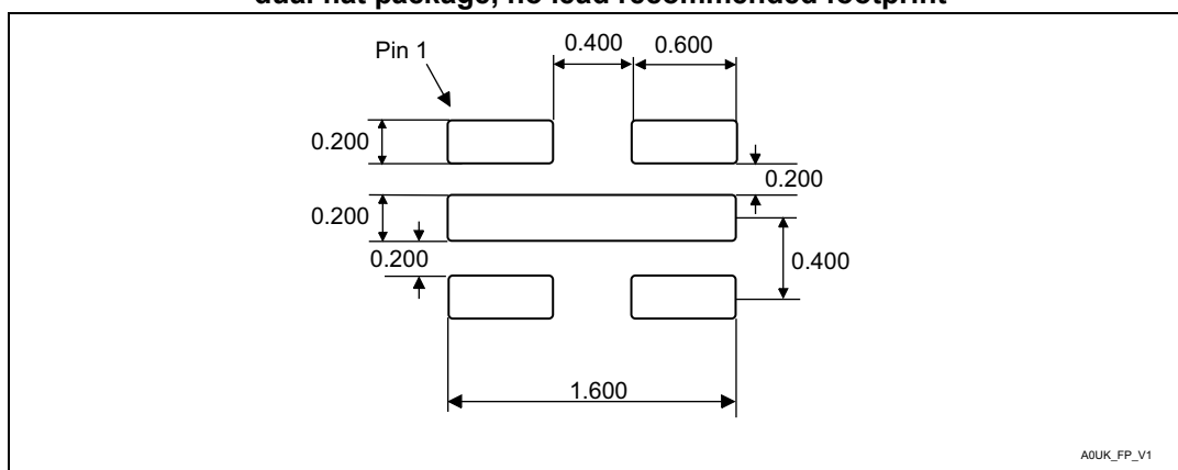
Figure 17. UDFFPN5 - 5-lead, 1.7 × 1.4 mm, 0.55 mm thickness, ultra thin fine pitch dual flat package, no lead recommended footprint
