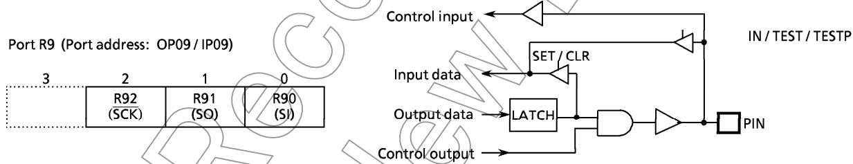
Figure 3-6. Port R9
