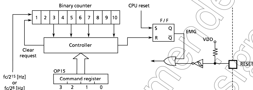
Figure 2-24. Configuration of Watchdog Timer
