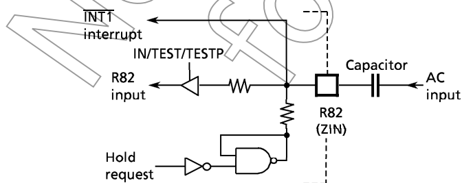
Figure 3-24. Zero-cross Detector
