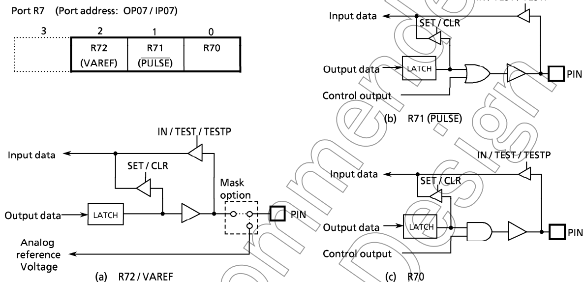
Figure 3-4. Port R7
