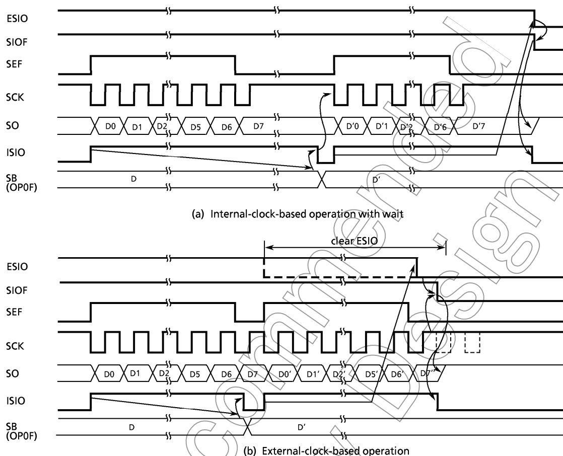
Figure 3-29. Transmit Mode
