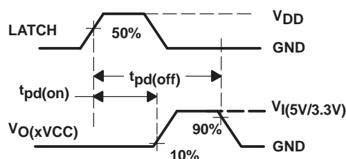
Propagation Delay (xVCC)
