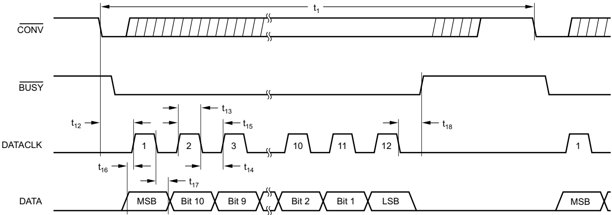
Figure 40. Serial Data Timing, Internal Clock ( \text{EXT}/\overline{\text{INT}} and \overline{\text{CS}} Low)
