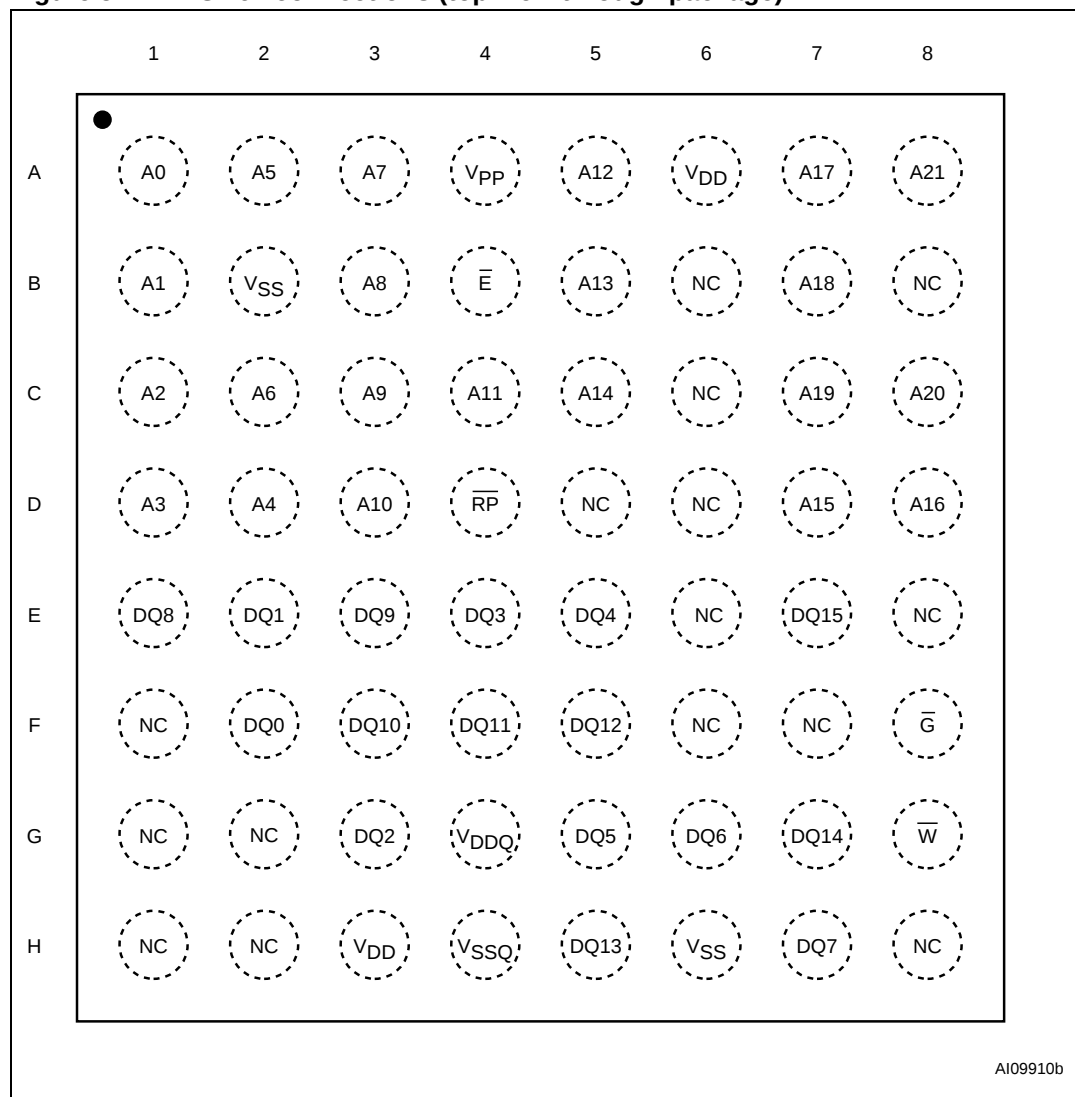
Figure 5. TBGA64 connections (top view through package)
