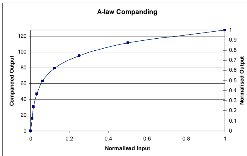
Figure 58 A-Law Companding
