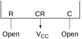
Figure 2 Oscillator Connection with HD61830
