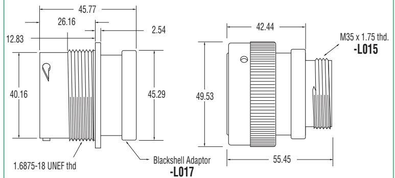
PLUG AND RECEPTACLE
