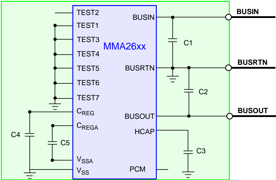
Figure 1. Application Diagram
