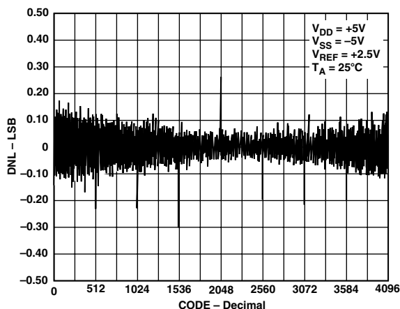
Figure 1. AD7398 DNL vs. Code ( T_A = 25^{\circ}\text{C} )
