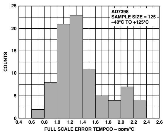
TPC 9. AD7398 Full-Scale Error Tempco
