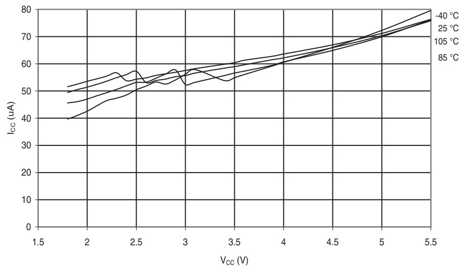
Figure 28-116. ATmega644P: Analog Comparator Current vs. V_{CC}
